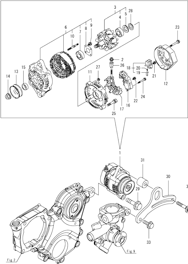
OCD50-M02790 ENGINE Fig.15. GENERATOR
